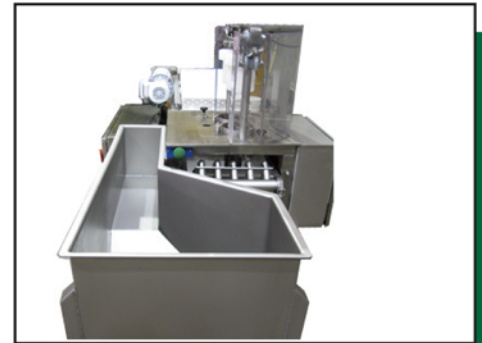
Pre-wash feed trough
