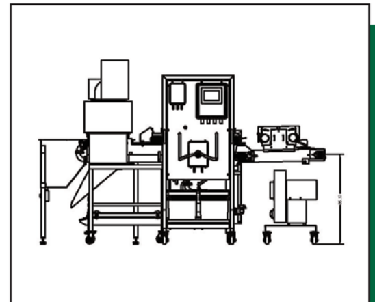
F2000AT with NatureSeal® monitor and control system
